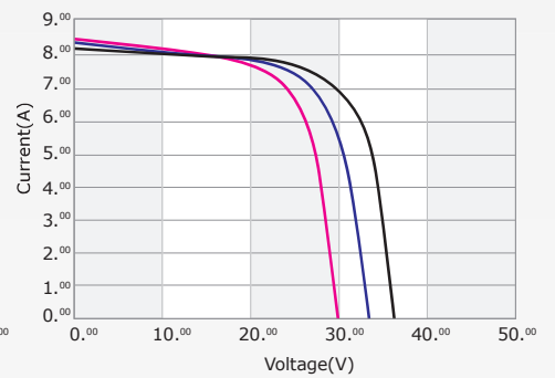
Temperature I-V Curves of TSM-D05-230
