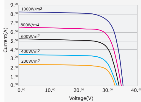
I-V Curves of TSM-D05-230
